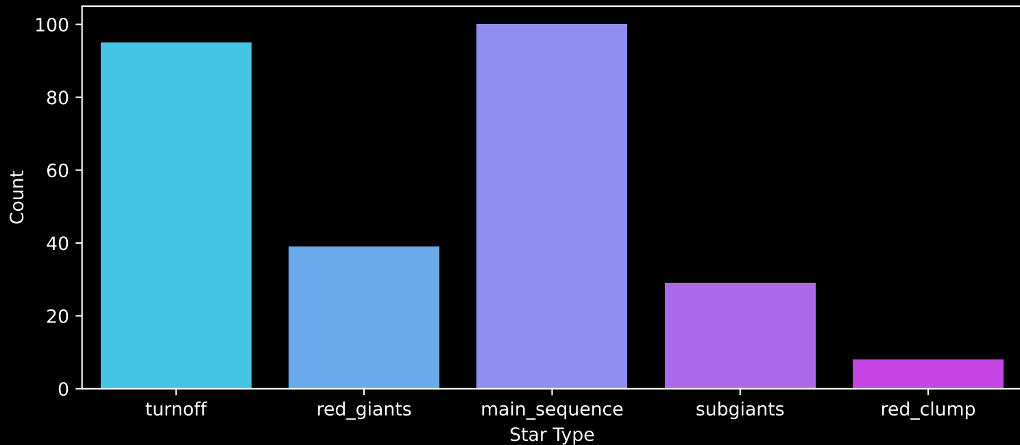
GALAH DR4 Field: [2439] Count plot of Star Type
