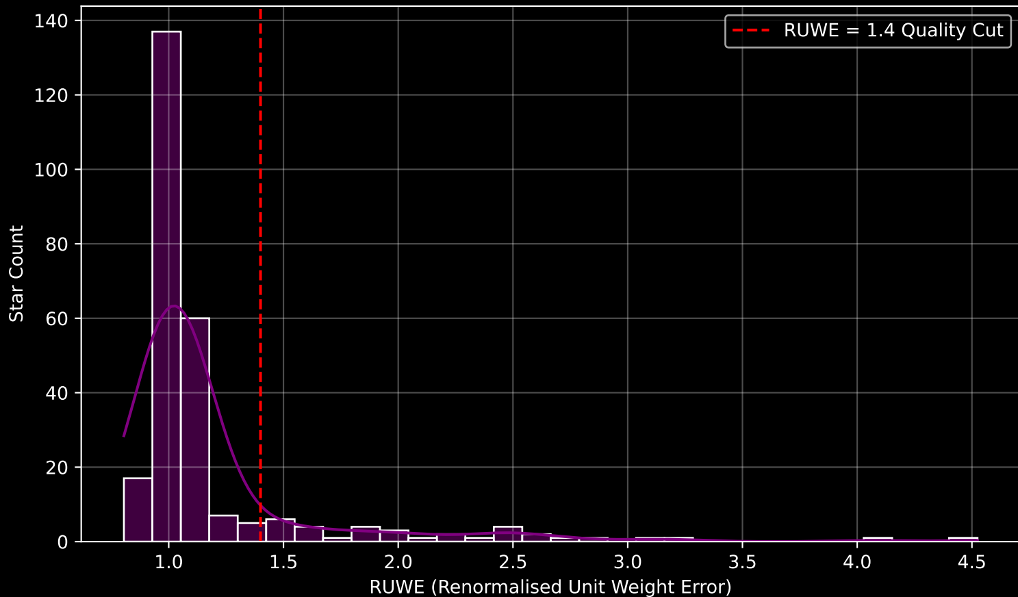
GALAH DR4 Field [2439] RUWE Distribution (n= 260)
