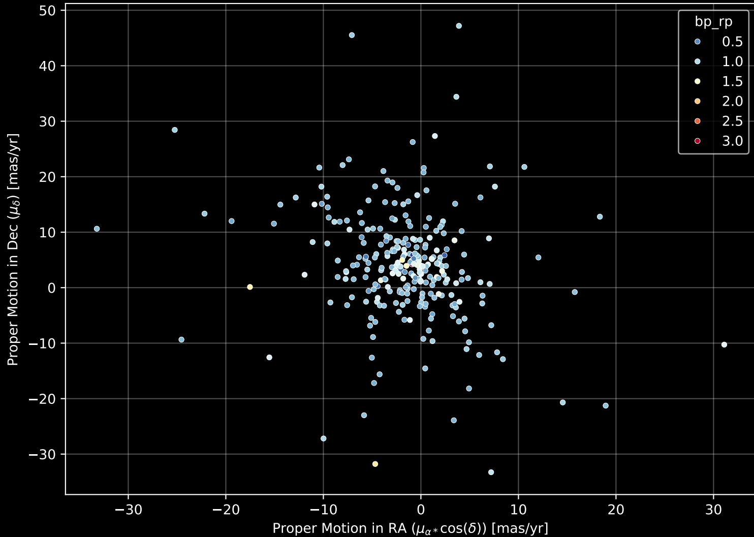
GALAH DR4 Field: [2439] Proper Motion Diagram (n= 271)
